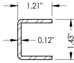
12 FIXED INTERLOCK (PD34) Roll formed steel
