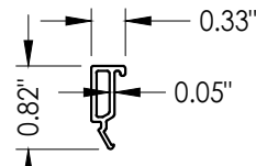
6 GLAZING BEAD Extruded vinyl
